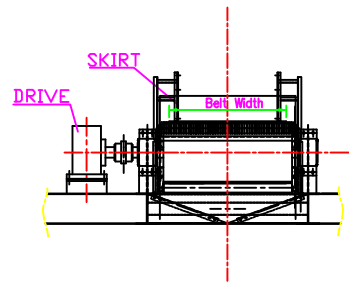
VIEW B-B
